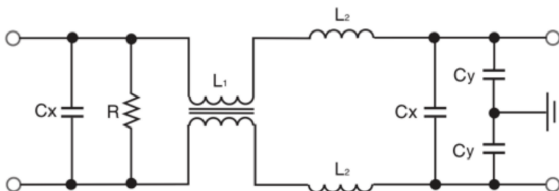
Figure 19: Typical structure of power supply EMC filters
